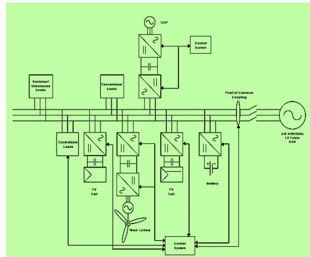
Fig. 1.1: Concept of a Micro grid
