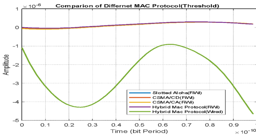
Figure 8. Comparison for threshold amplitude
