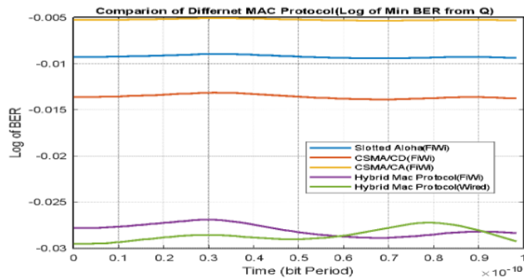
Figure10. Comparison graph for BER from Q Factor
