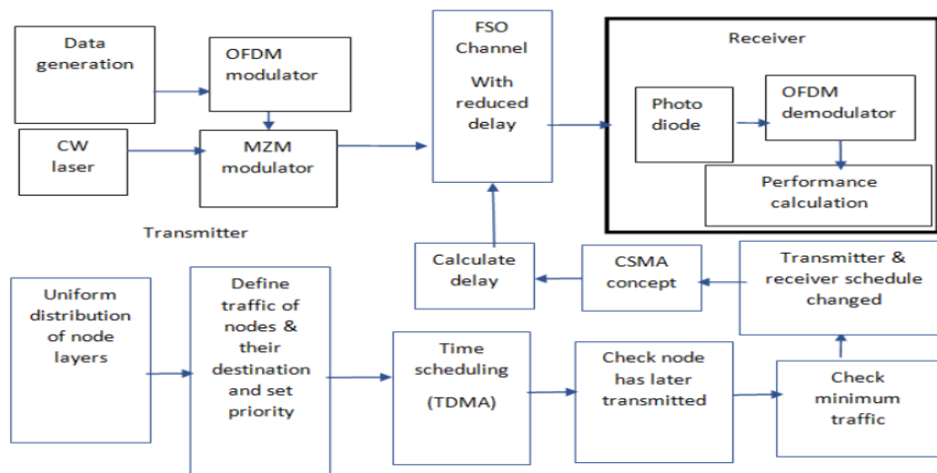
Figure 2. Proposed MAC protocol model
