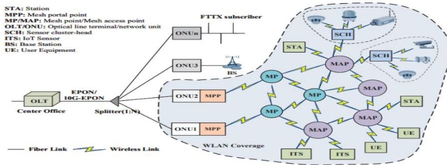
Figure 1. General architecture of Fi-Wi networks
