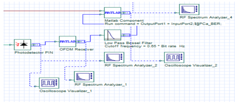
Figure 5. Receiver channel of proposed approach
