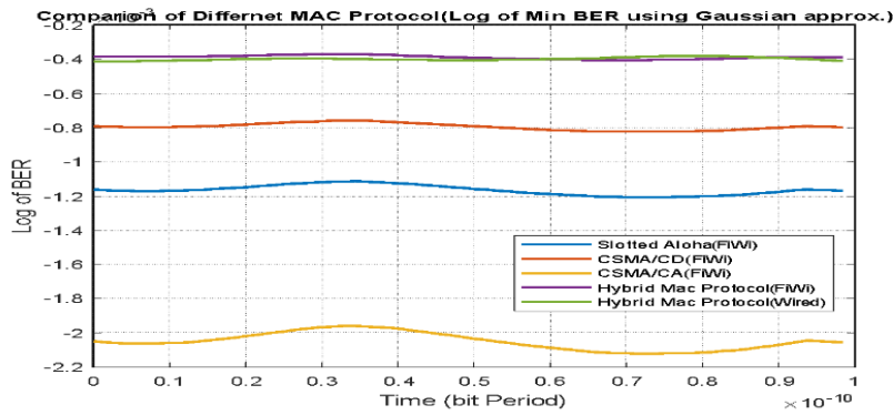
Figure 9. Comparison graph for BER using Gaussian approx
