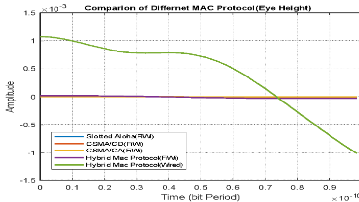
Figure 7. Comparison for Eye pattern Diagrams
