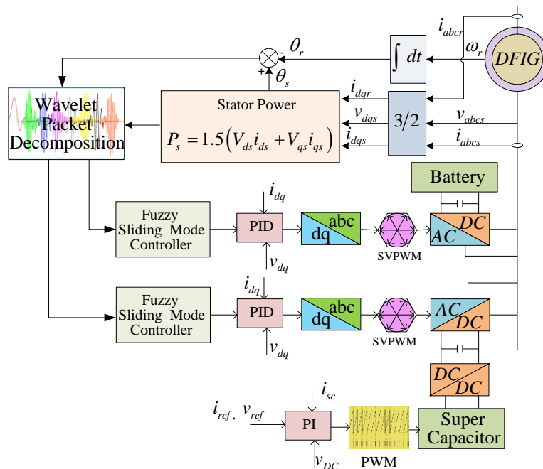
Fig. 3 Diagram of Dual-energy control system
