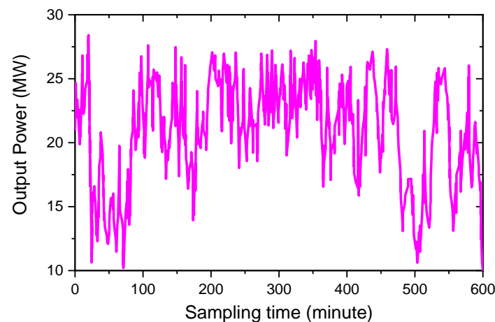
Fig. 8 Curve of wind output power
