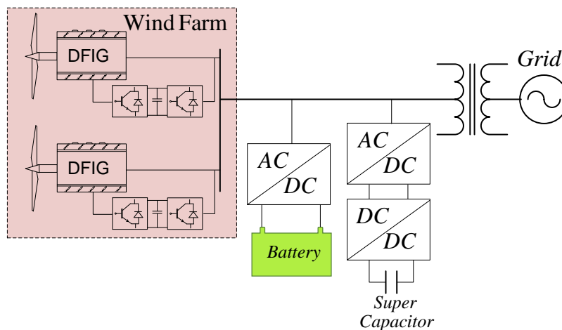
Fig. 1 DFIG system with Dual energy system
