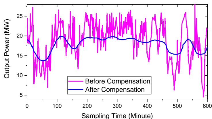
Fig. 10 DFIG output power
