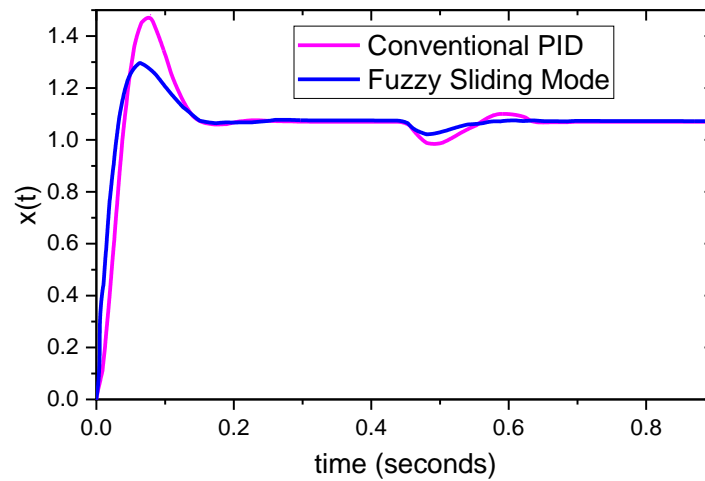
Fig. 7 Fuzzy sliding and PID system response comparison
