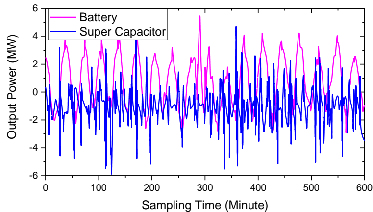
Fig. 12 Battery and super-capacitor power
