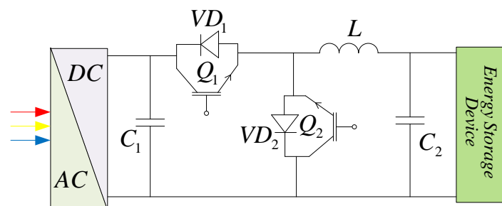
Fig. 2 Boost converter: DC/DC bidirectional
